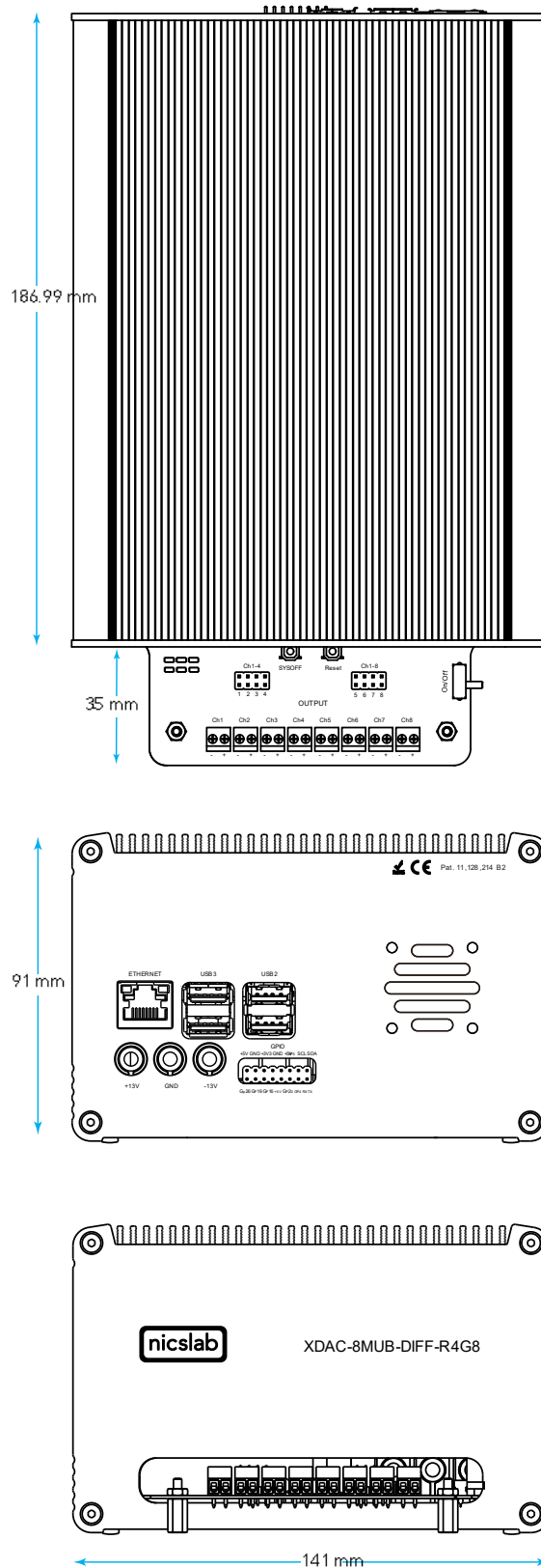
Figure 2. Product Dimension
