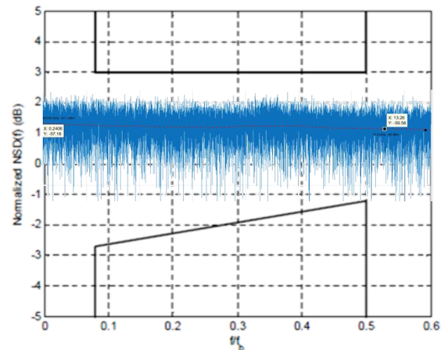
Figure 13: Noise Flatness
